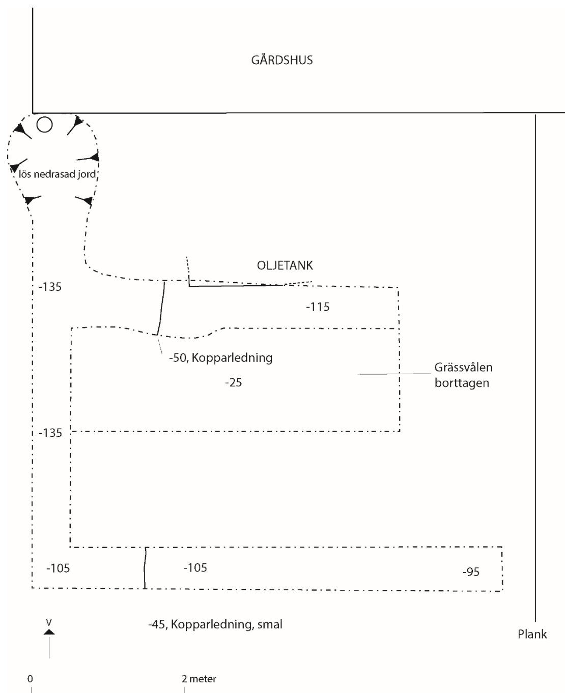
Figur 3. Schaktplan.
